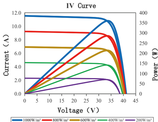
Current-Voltage & Power-Voltage Curve
