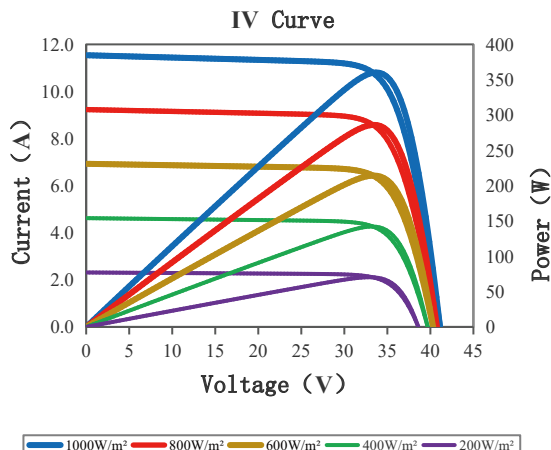
Current-Voltage & Power-Voltage Curve
